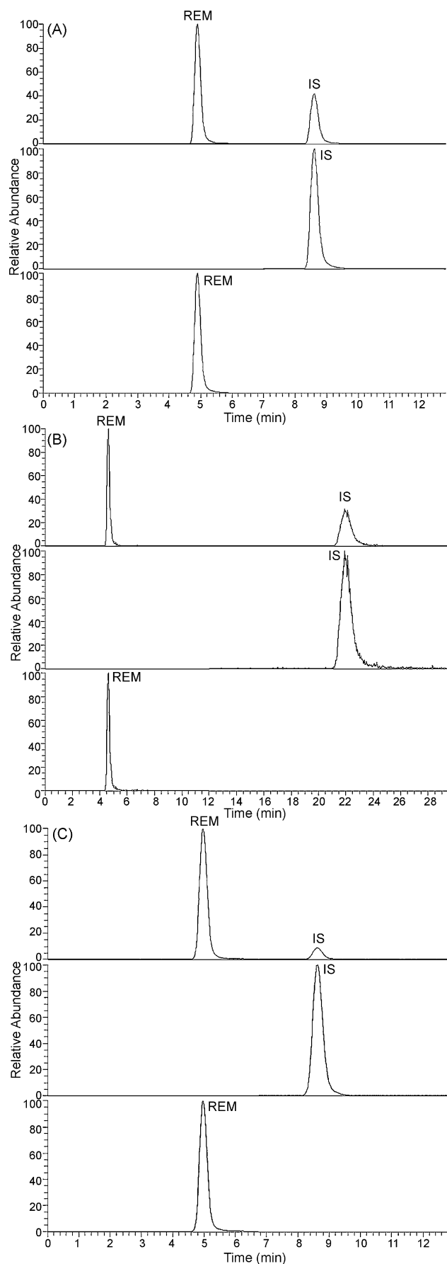
Fig. 2. Relative abundances of remoxipride (REM) and raclopride (IS) in different matrices in an individual rat after administration of 16 mg/kg remoxipride at t=0 . The upper panel shows the chromatogram of the sample. The lower panels show the peaks of the IS (middle panel) and remoxipride (lower panel) within that sample. (A) Chromatograms of plasma sample at t=40 min, (B) chromatograms of microdialysate sample at t=140 –160 min and (C) chromatograms of a brain homogenate sample at t=240 min.
