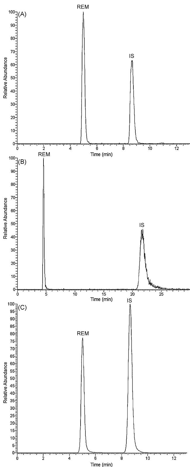
Fig. 1. Relative abundances of remoxipride (REM) and raclopride (IS) in different matrices. (A) Chromatogram of plasma spiked with 20 ng/ml remoxipride, (B) 2 ng/ml remoxipride in microdialysate and (C) 20 ng/ml remoxipride in brain homogenate.
